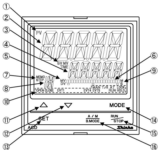
ACD-15A
