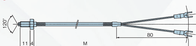
形名: PS-C (熱電対) Model: PS-C (Thermocouple)
