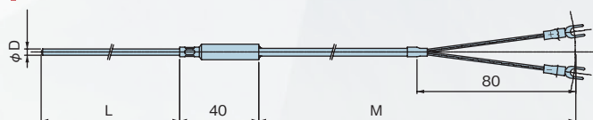
形名: PC-B (TC-S) (シース熱電対), PC-BR (シース測温抵抗体) Model: PC-B (TC-S) (Sheath thermocouple), PC-BR (Sheath RTD)
