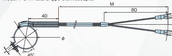
形名: PC-RT (バンド形熱電対) Model: PC-RT (Band type thermocouple)
