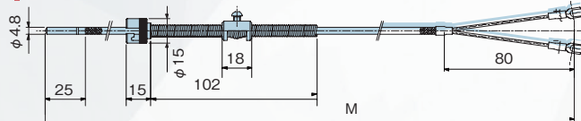
形名: PC-SH (摺動圧接形) (熱電対) Model: PC-SH (Pressure sliding type) (Thermocouple)
