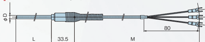
形名: PC-B (熱電対), PC-BR (測温抵抗体) Model: PC-B (Thermocouple), PC-BR (RTD)
