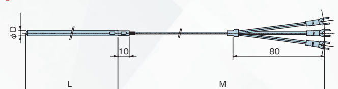
形名: NR-100-P (測温抵抗体) Model: NR-100-P (RTD)
