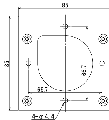
Mounting Plate
