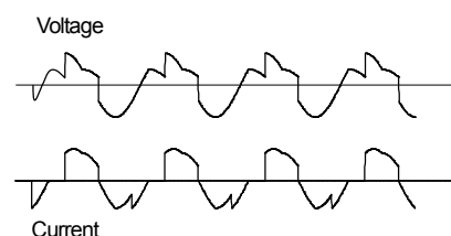
[3-arm control waveform]
