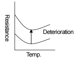
Silicon carbide (SiC) heater
