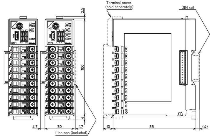
Control Module QTC1-2/QTC1-4
