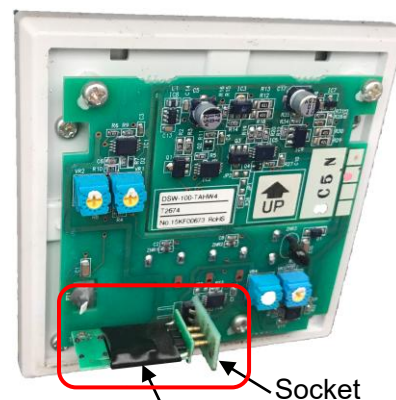
Humidity sensor (HD-S2)
