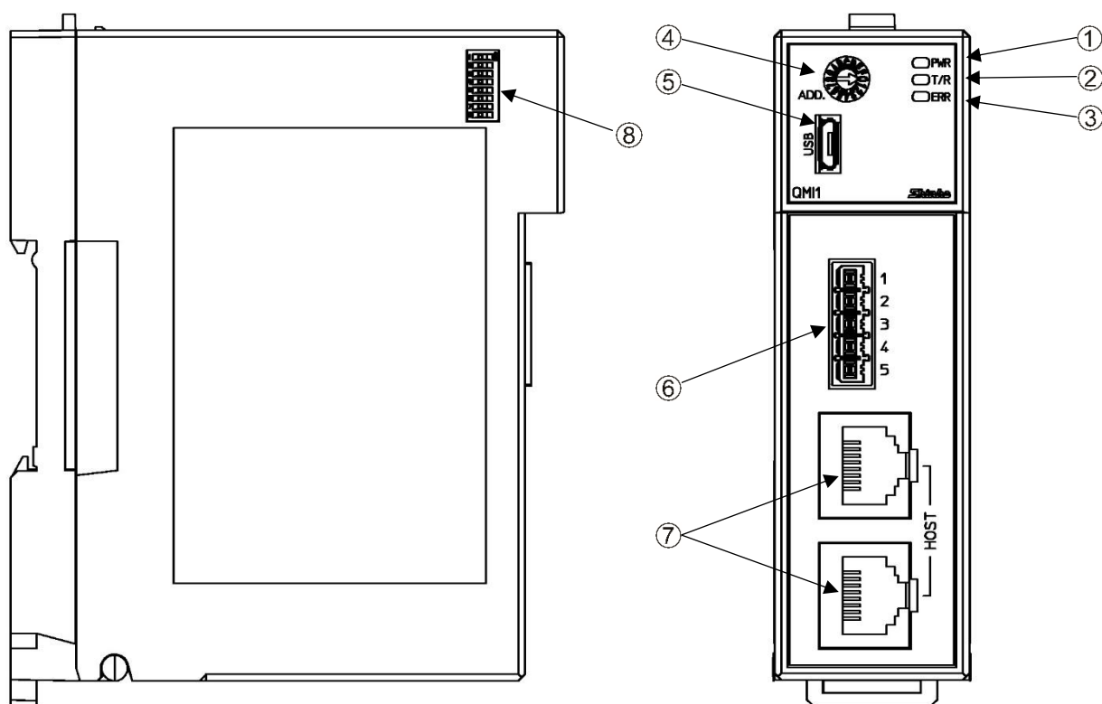
Base part
