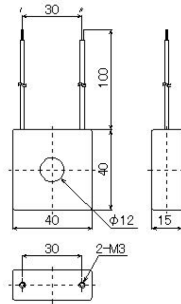
CTL-12-S36-10L1U(100 A 用)
