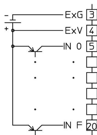
RG-CU-DI32B (PNP)
