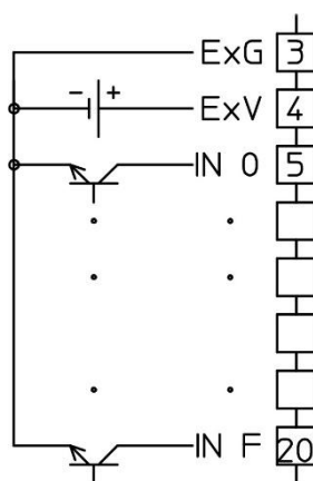
RG-CU-DI32A (NPN)
