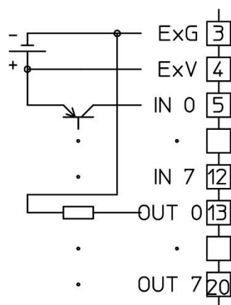
RG-CU-DIO8B (PNP)
